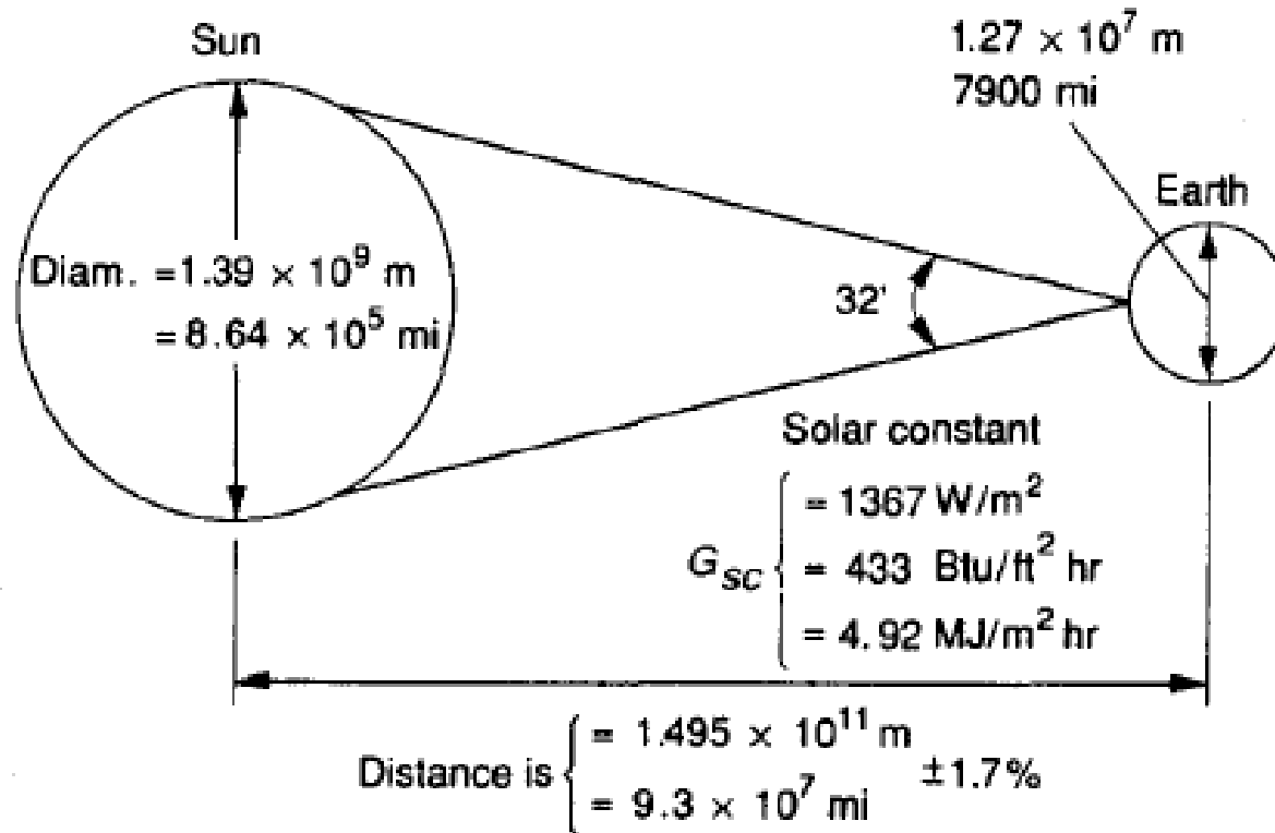
Figure 1.2.1 Sun-earth relationships.
