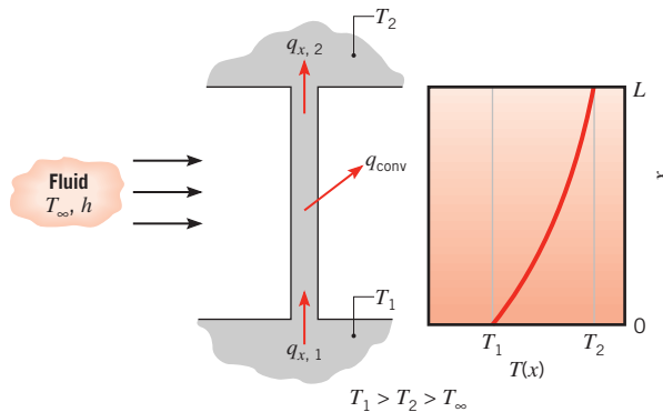
FIGURE 3.12 Combined conduction and convection in a structural element.
