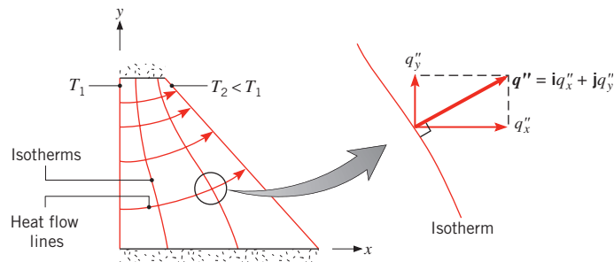
FIGURE 4.1 Two-dimensional conduction.
