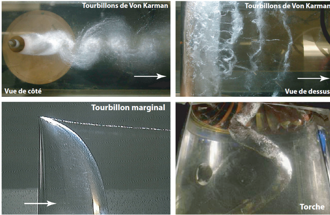
Figure 1.4 – La cavitation de vortex
