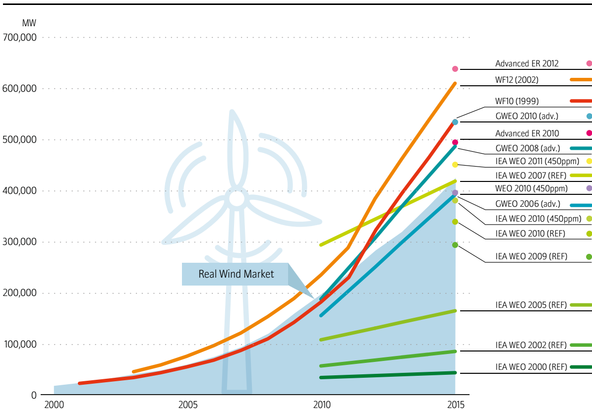
Figure 16: Wind power projections versus real market developments
