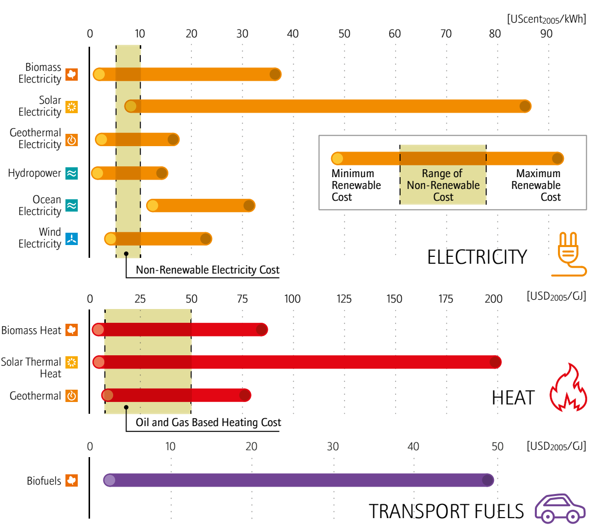
Figure 31: Range of levelised costs of energy for selected commercially available renewable energy technologies compared to non-renewable energy costs – cost development, 2010 – 2015
