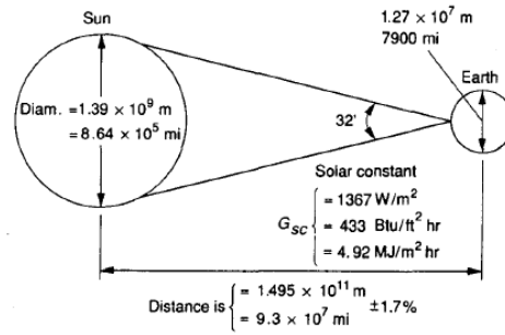
Figure 1.2.1 Sun-earth relationships.
