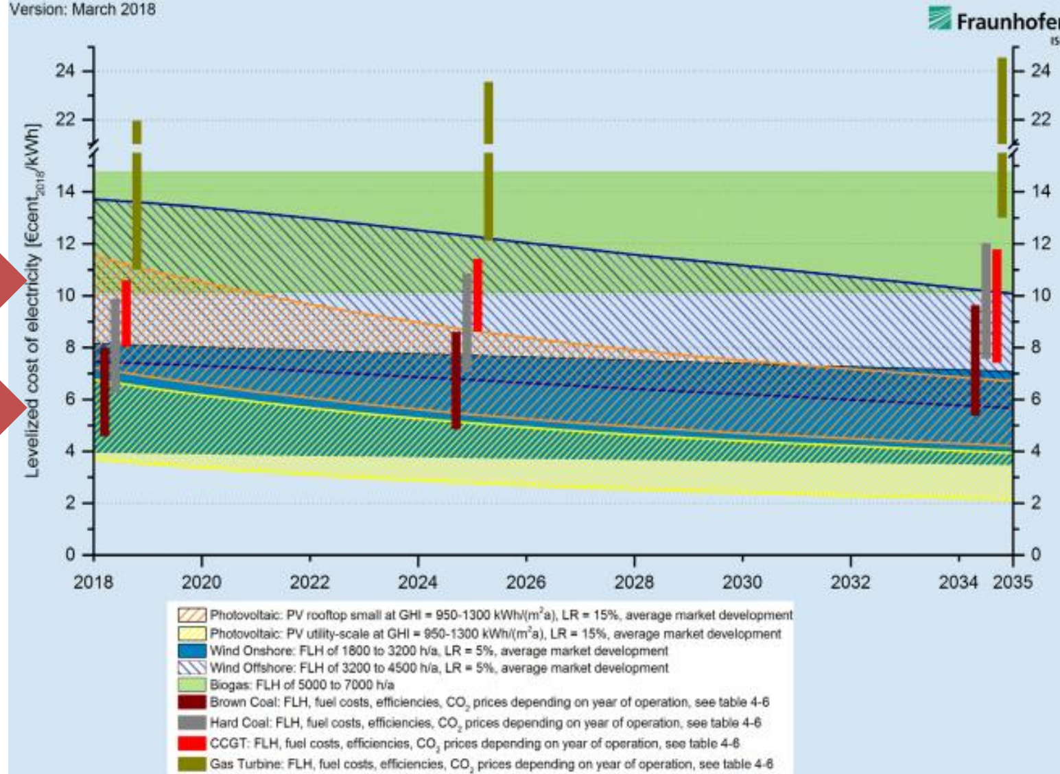
EN2018_Fraunhofer-ISE_LCOE_Renewable_Energy_Technologies March 2018
